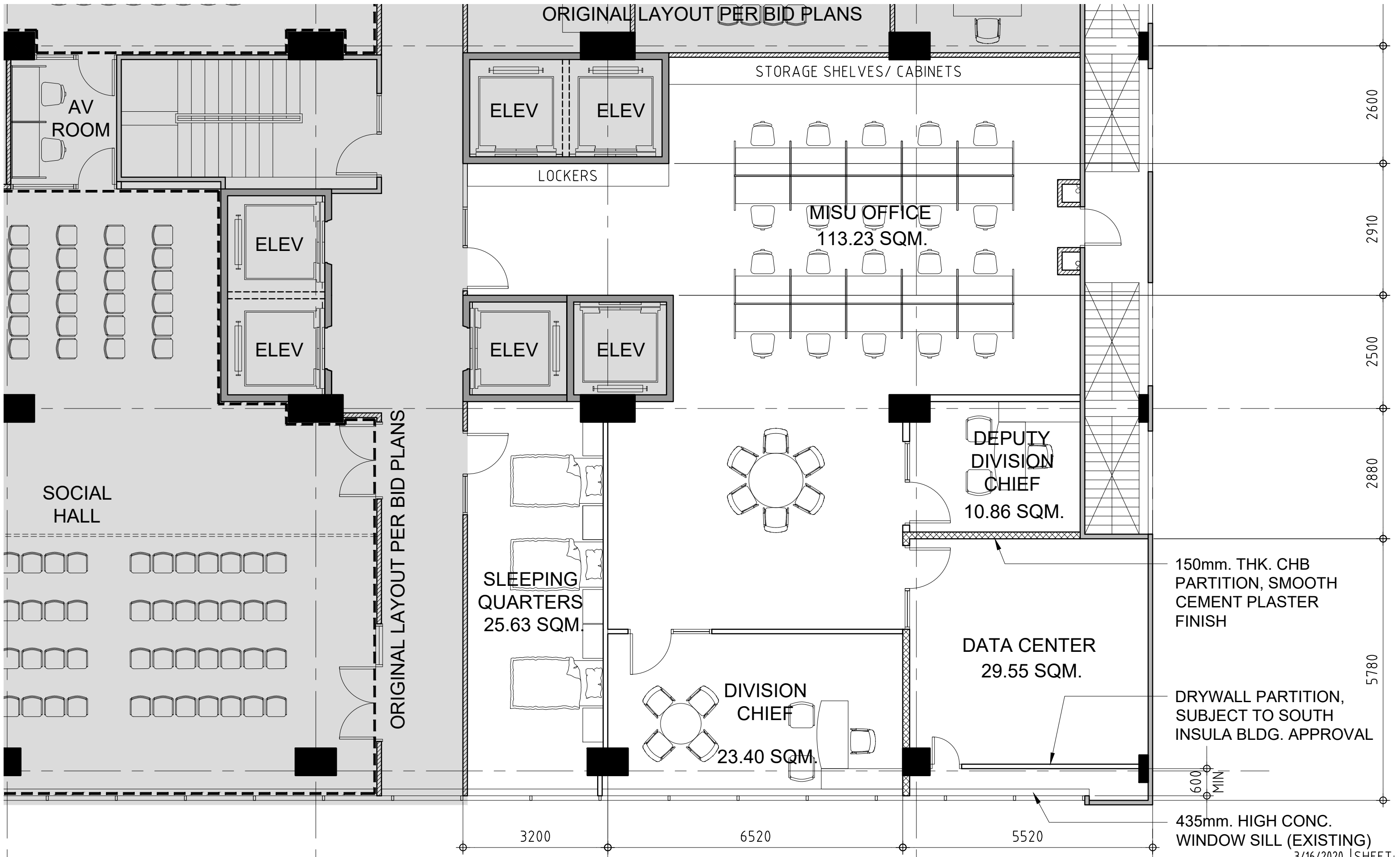
1 PARTIAL PLAN SK-3 SCALE 1: 75 M.
